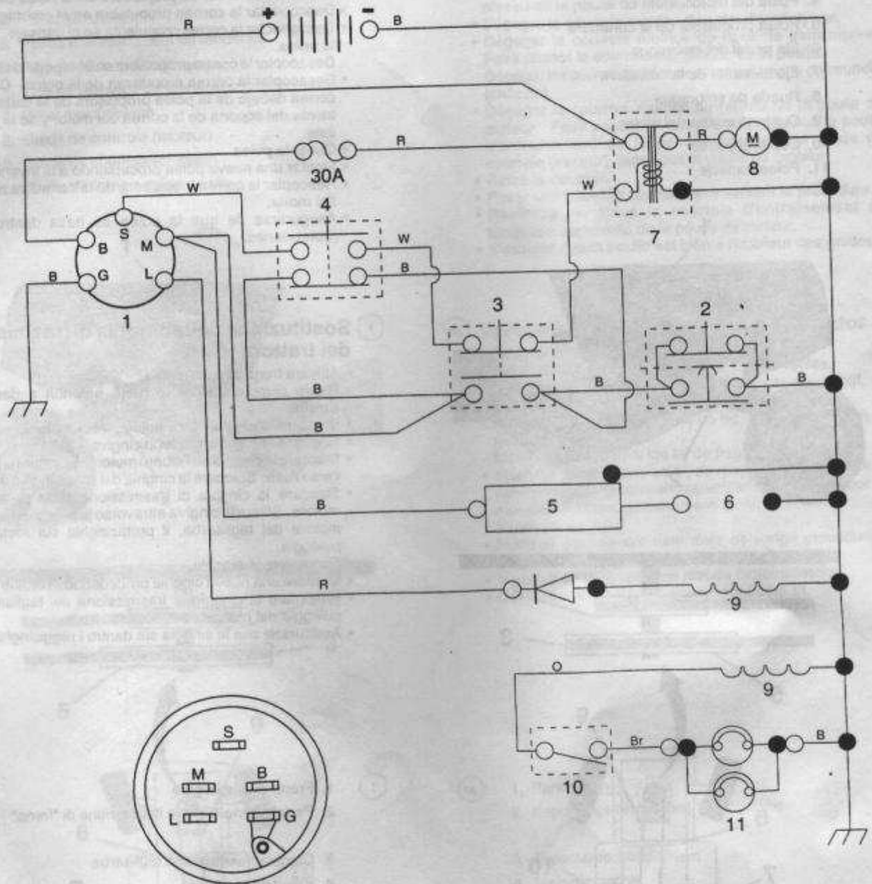
Ignition switch
