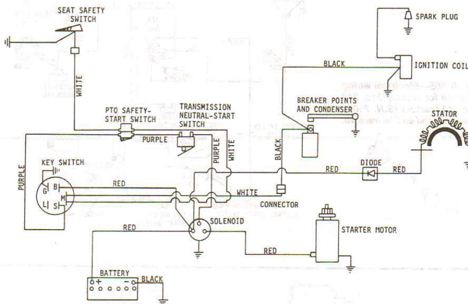
Fig. JD102—Electrical wiring diagram for Models 108 and 111 tractors (S.N. 120001 and later).
