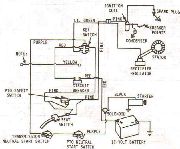
Fig. JD103—Electrical wiring diagram for Model 208.
