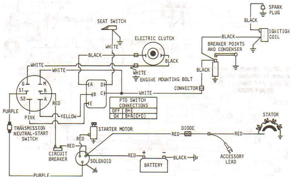
Fig. JD101—Electrical wiring diagram for Models 108 and 111 tractors (S.N. 95001-120000).
