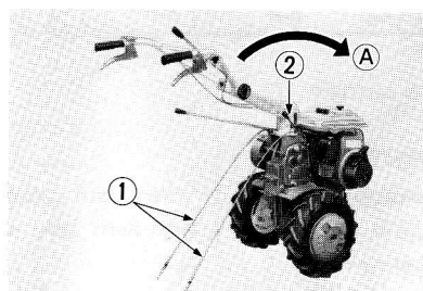
① Steering clutch wires
