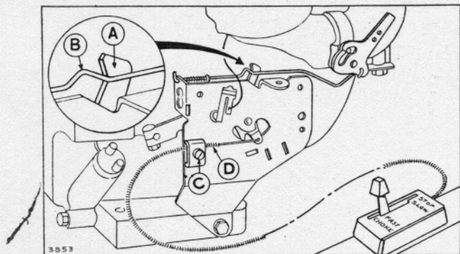
Fig. 4 - Choke-A-Matic Control (Typical)
