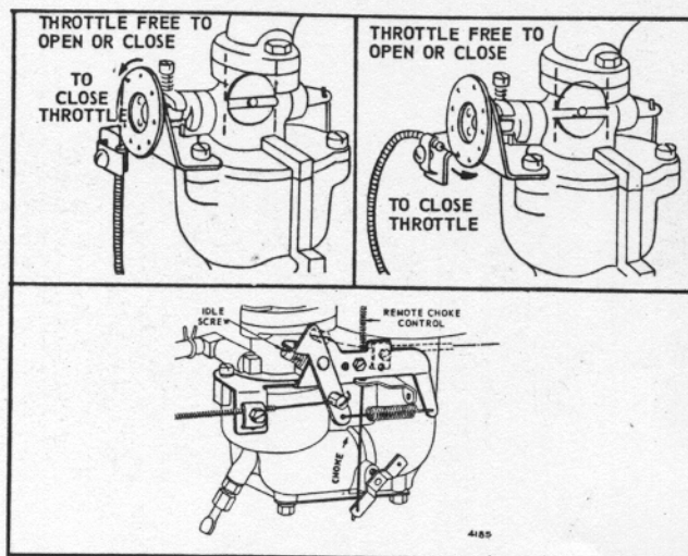
Fig. 2 - Remote Throttle Control
