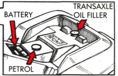
LIFT SEAT OFF FOR ACCESS.
