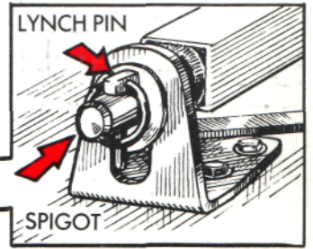
CUTTER DECK FRONT SUPPORT BRACKET SHOWING SPIGOT AND LYNCH PIN.
