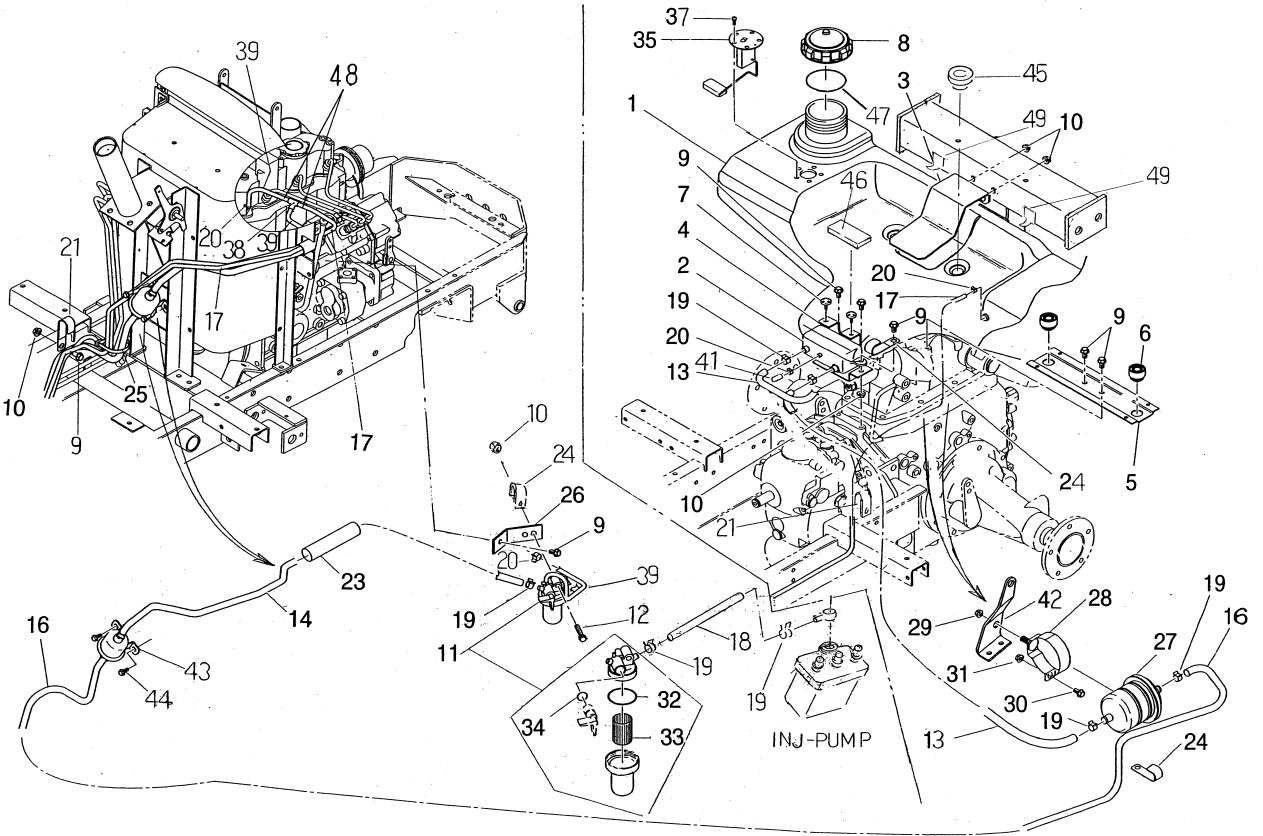
FIG.228 FUEL TANK
