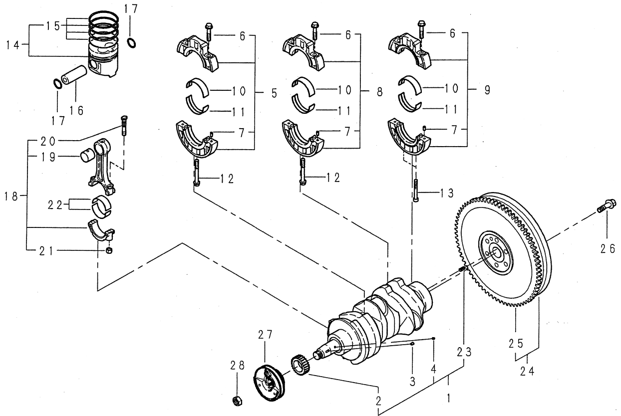
FIG.106 CRANK SHAFT,PISTON
