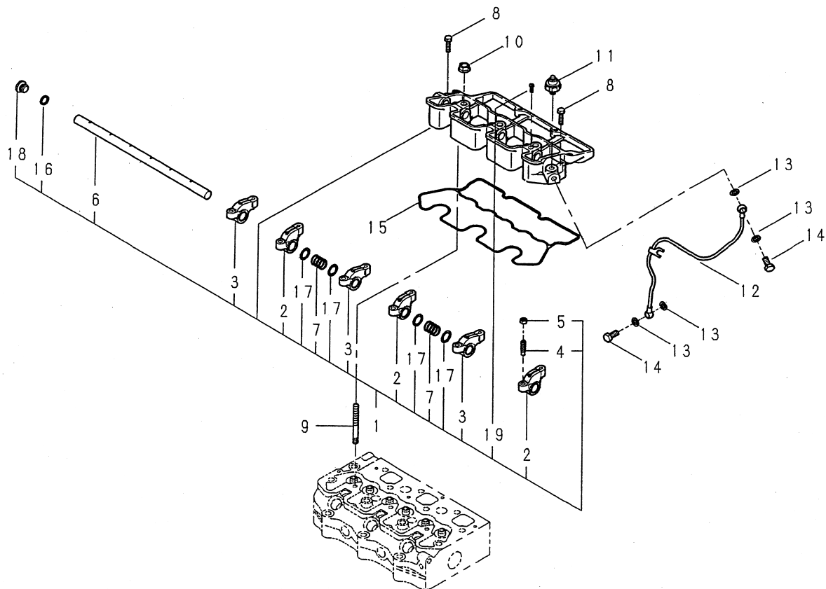
FIG.104 ROCKER ARM ASSY
