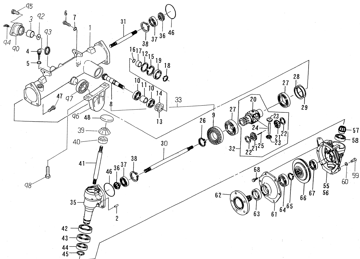
FIG.201 FRONT UNIT
