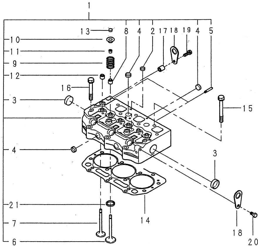
FIG.103 CYLINDER HEAD
