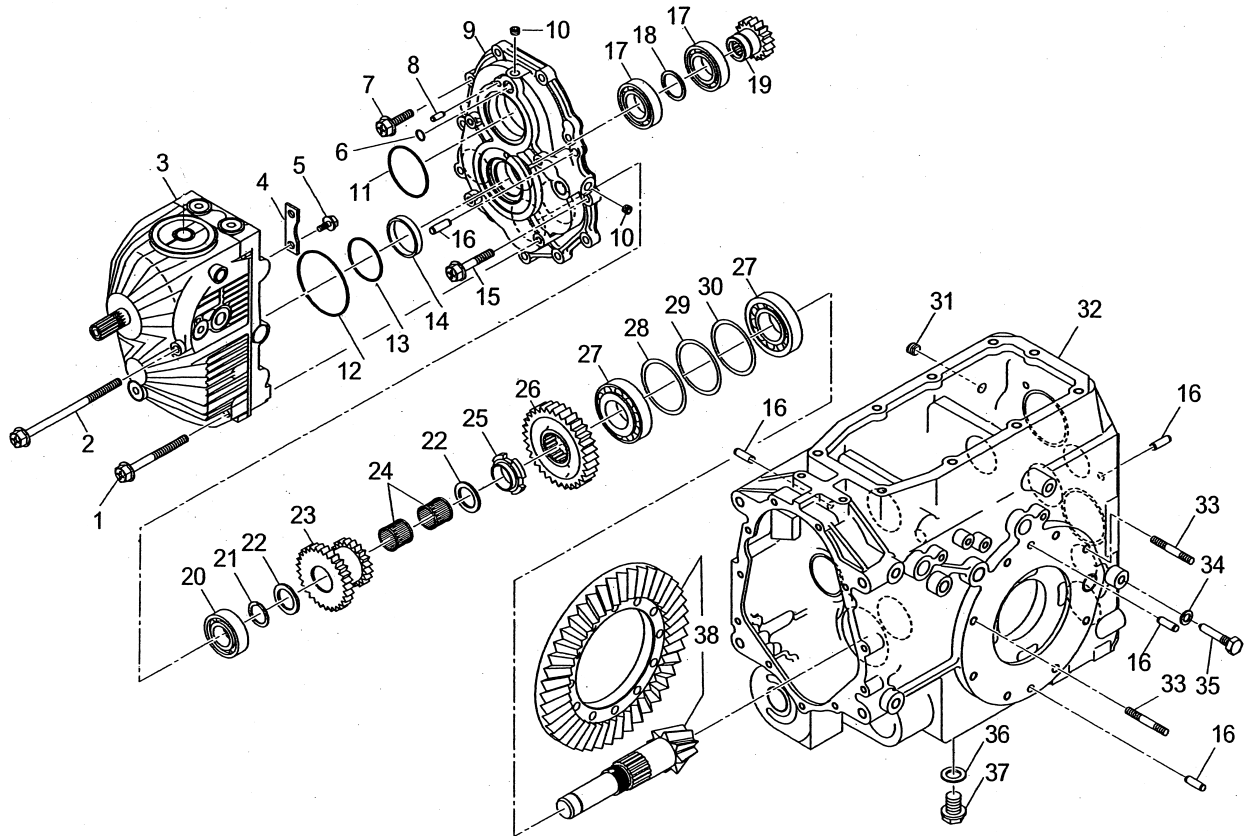
FIG.207 MISSION ; DRIVE
