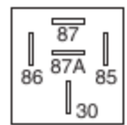
RELAY
