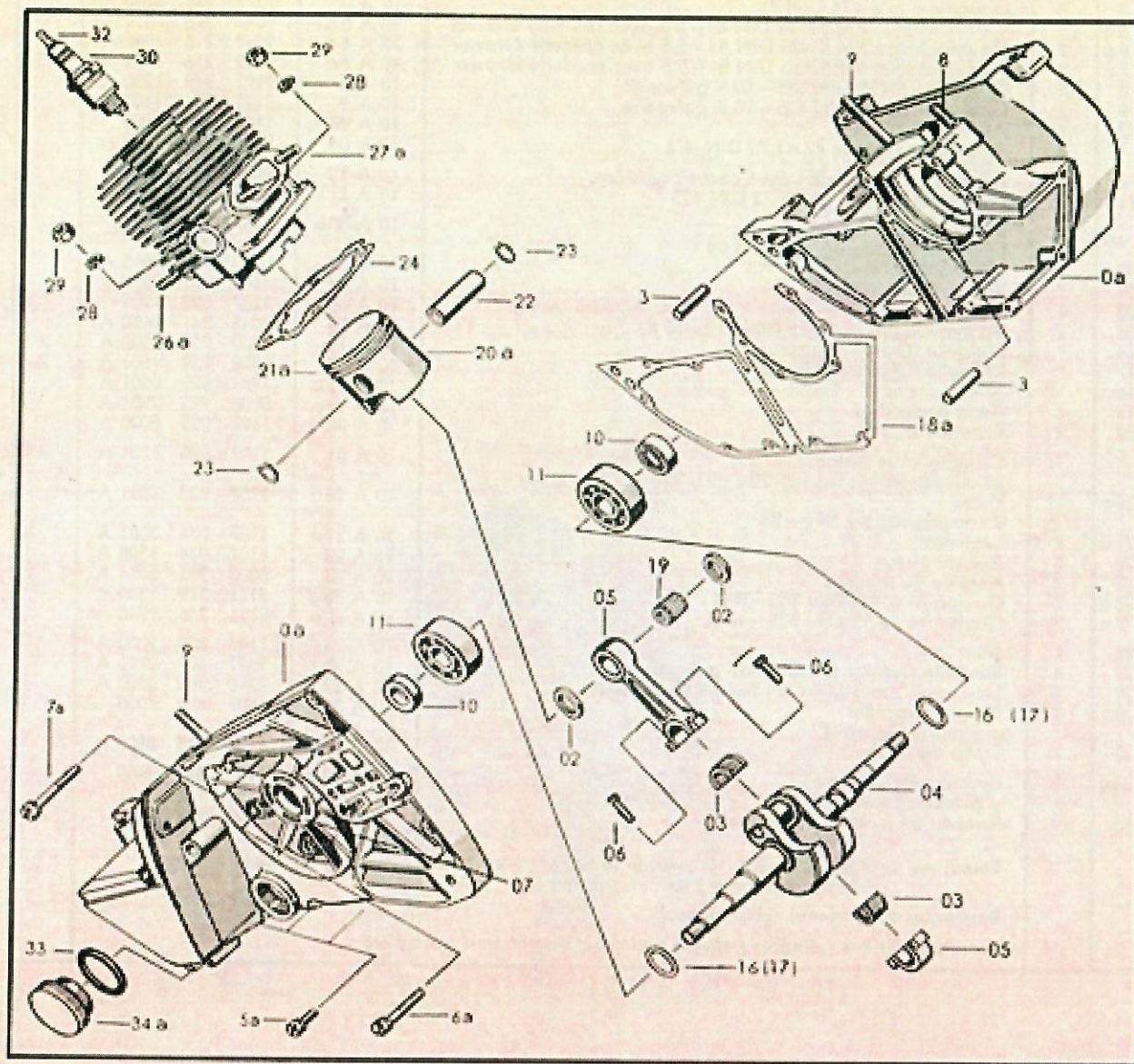
Illustration A Carter, Vilebrequin, Paliers, Piston, Cylindre
